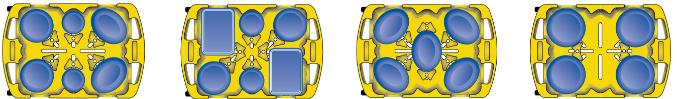
ADD6 Layout for 30,5cm by 23cm to 24cm by 18,5cm platters, 14cm to 20cm plates and 14cm to 30,5cm plates ADD6 Layout for 25,5cm by 37cm trays and 19cm plates and 25,5cm plates ADD6 Layout for 30,5cm by 23,5cm to 24cm by 18,5cm platters ADD4 Layout for 29cm to 32cm plates and 34cm by 26,5cm platters
